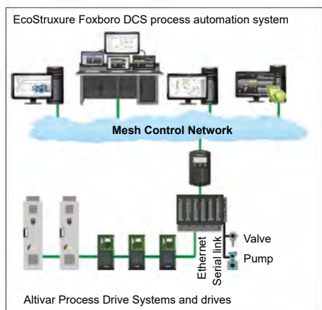
Altivar Process Drive Systems and drives in EcoStruxure Foxboro DCS architecture
