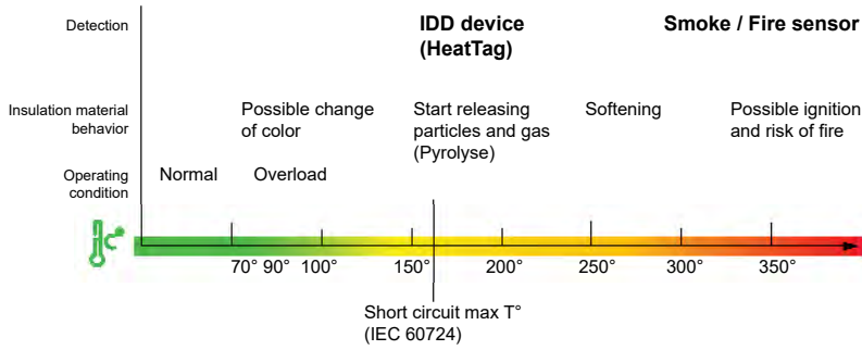
PVC insulation material behavior with increasing temperature
