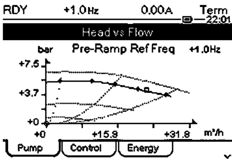
Pump monitoring display
