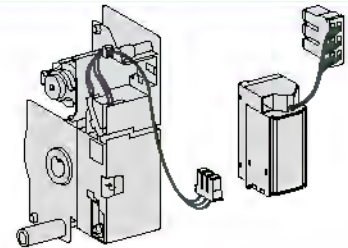
Gear motor
