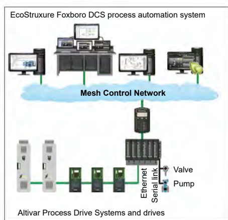
Altivar Process in EcoStruxure Foxboro DCS architecture
