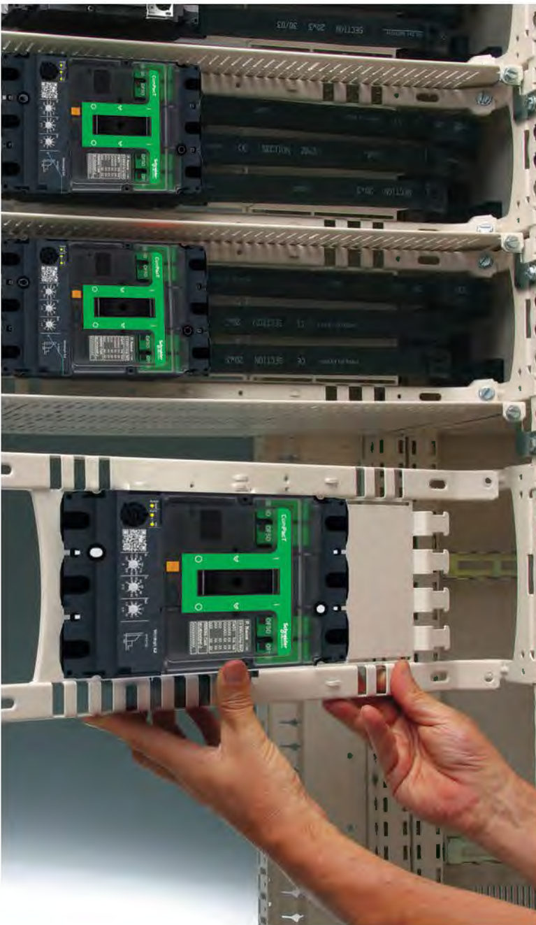
Temperature rise test in laboratory.
