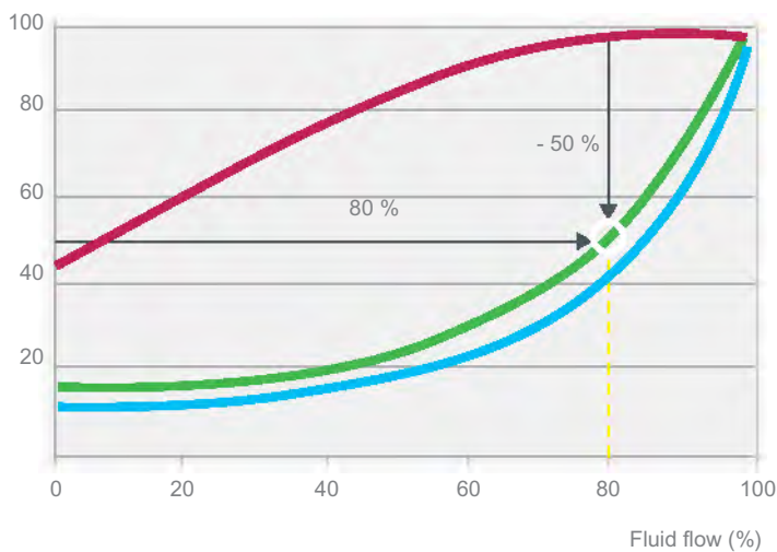
Power consumption (%)
