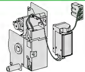
Gear motor
