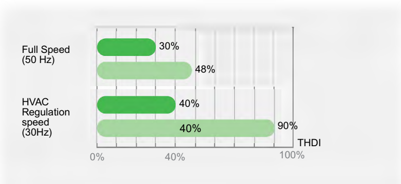
■ Altivar 212 antiharmonic technology ■ Drives with integrated DC choke
